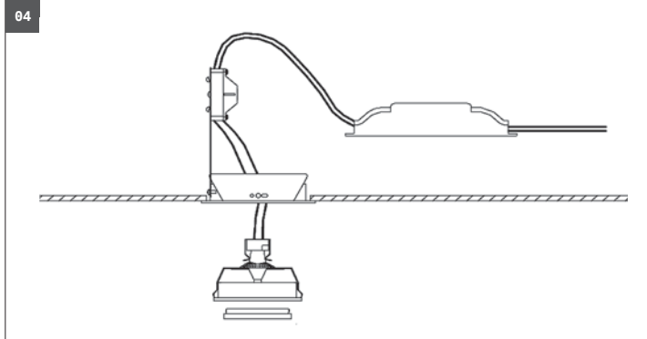
Screw cover ring and mounting frame together.
