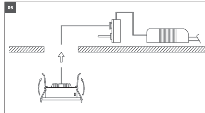
Compress the cramp at the downlight back...
