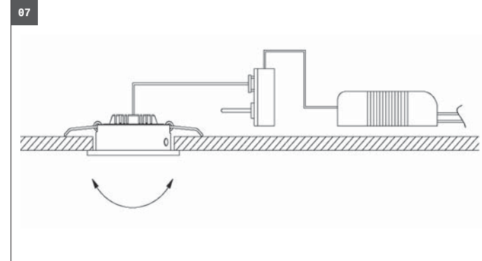
...include the downlight in the ceiling cutout, to secure release the cramp.
