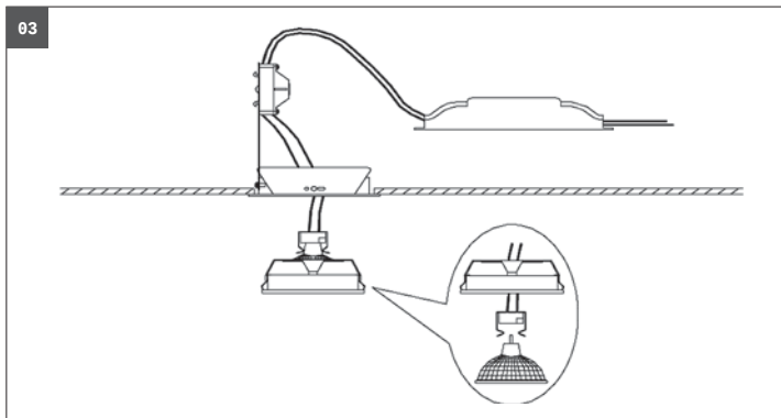
Insert the luminaire (not included in delivery) in the socket. Insert the downlight in the mounting frame.
