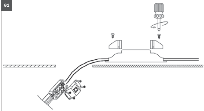
Connected cable with transformer (not included in delivery).
